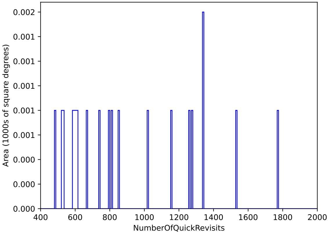
ddf_acor_sf15_lsf20_lsr20_v3.4_10yrs WFD: NumberOfQuickRevisits
