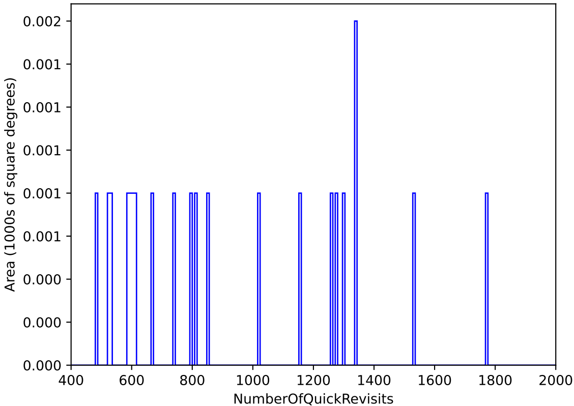
ddf_acor_sf15_lsf20_lsr20_v3.4_10yrs All sky: NumberOfQuickRevisits
