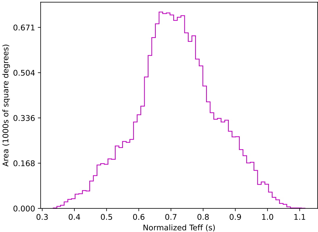
ddf_acor_sf15_lsf20_lsr20_v3.4_10yrs WFD z band: Normalized Teff
