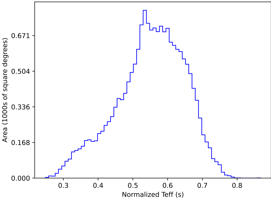
ddf_acor_sf15_lsf20_lsr20_v3.4_10yrs WFD y band: Normalized Teff
