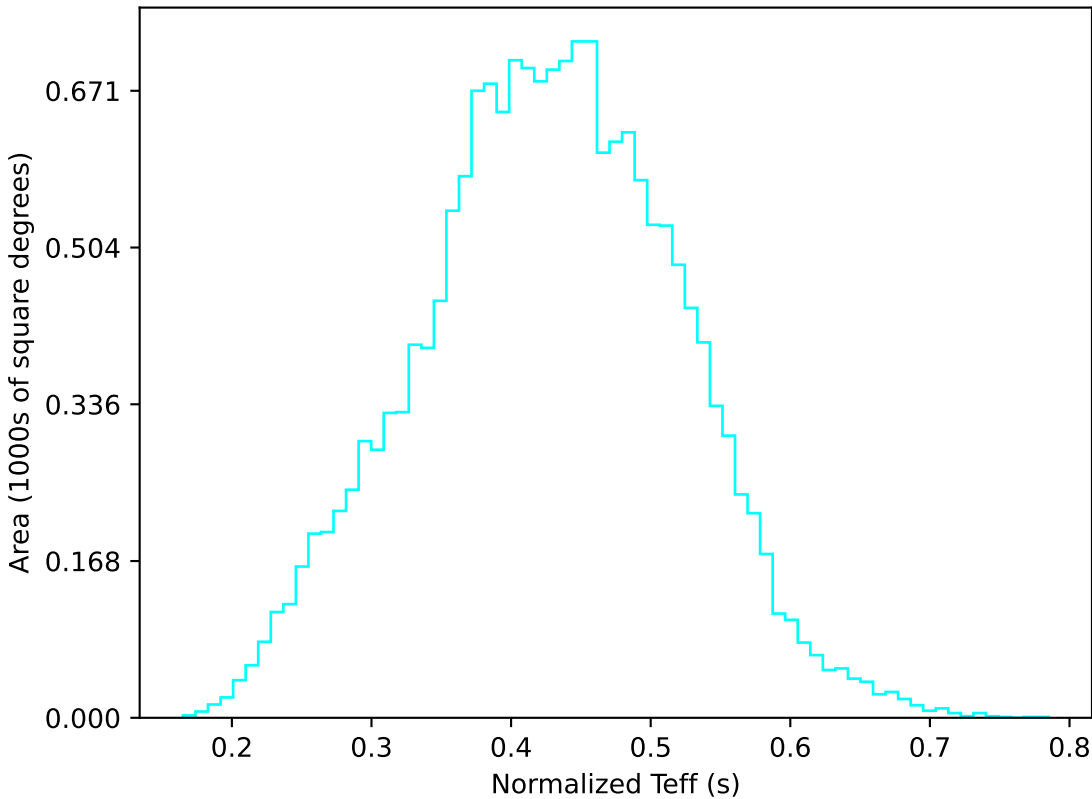
ddf_acor_sf15_lsf20_lsr20_v3.4_10yrs WFD u band: Normalized Teff
