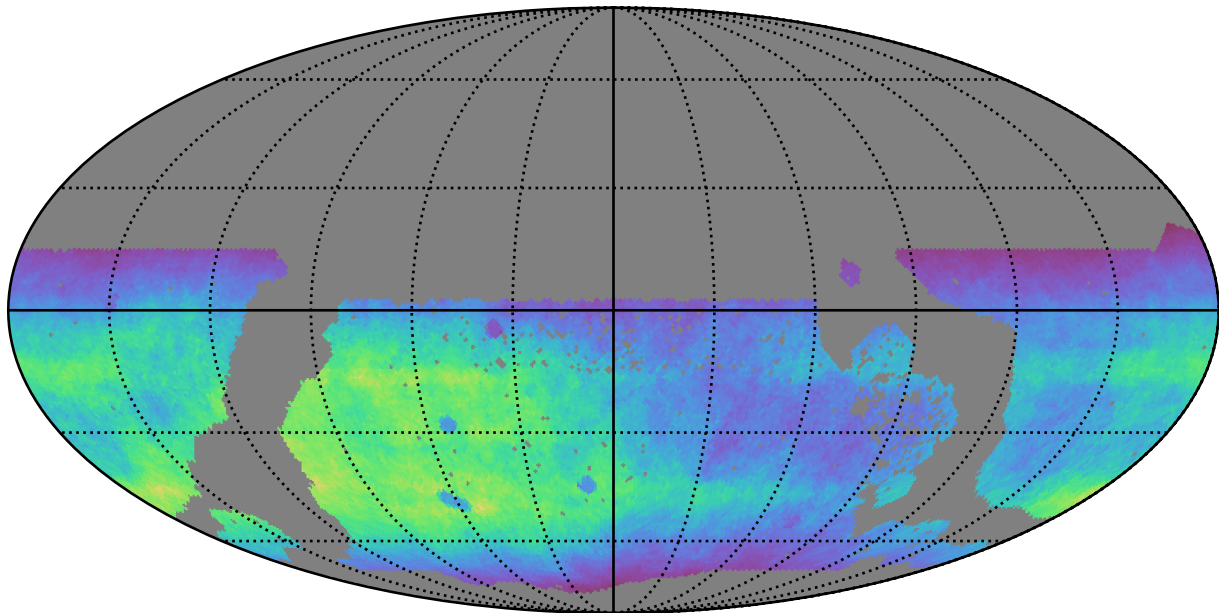
ddf_acor_sf15_lsf20_lsr20_v3.4_10yrs WFD r band: Normalized Teff
