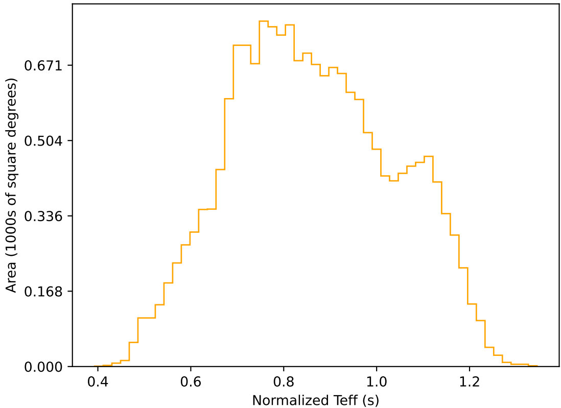
ddf_acor_sf15_lsf20_lsr20_v3.4_10yrs WFD r band: Normalized Teff
