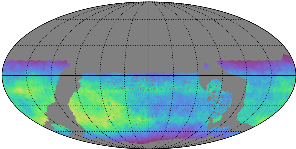
ddf_acor_sf15_lsf20_lsr20_v3.4_10yrs WFD i band: Normalized Teff
