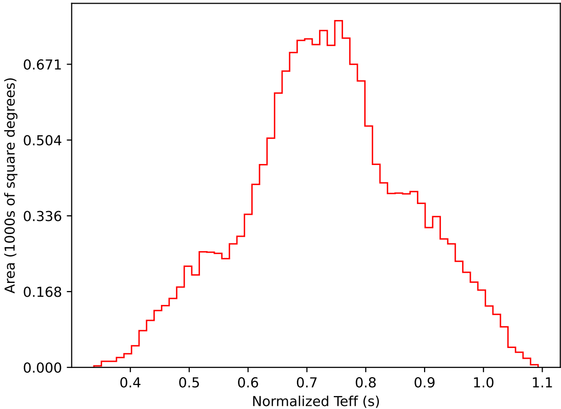
ddf_acor_sf15_lsf20_lsr20_v3.4_10yrs WFD i band: Normalized Teff
