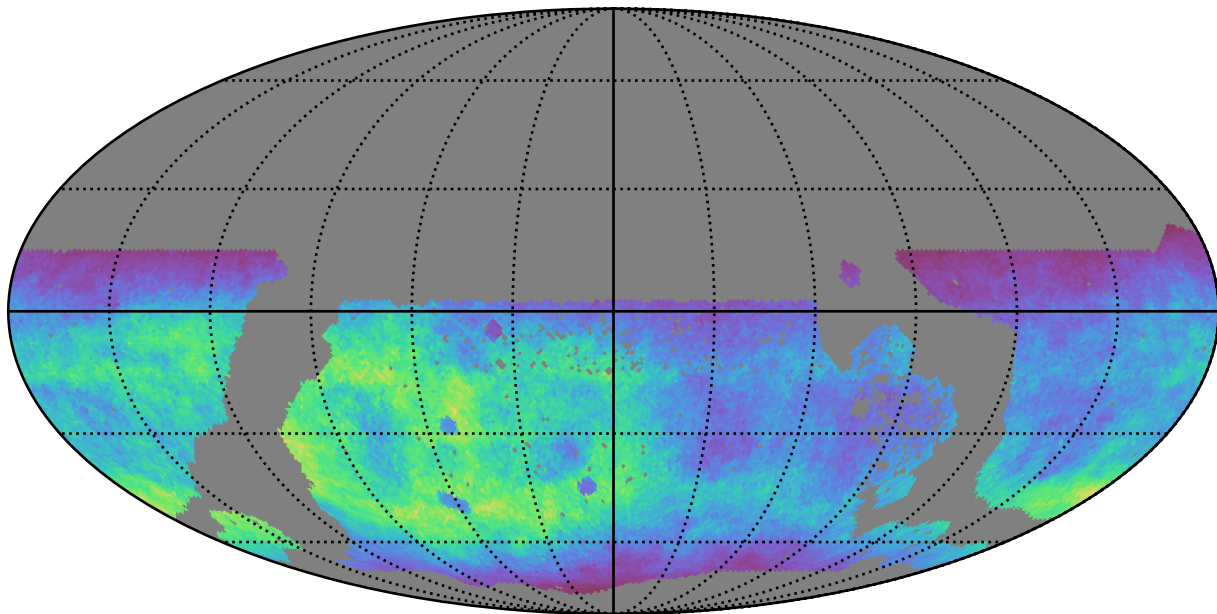
ddf_acor_sf15_lsf20_lsr20_v3.4_10yrs WFD g band: Normalized Teff
