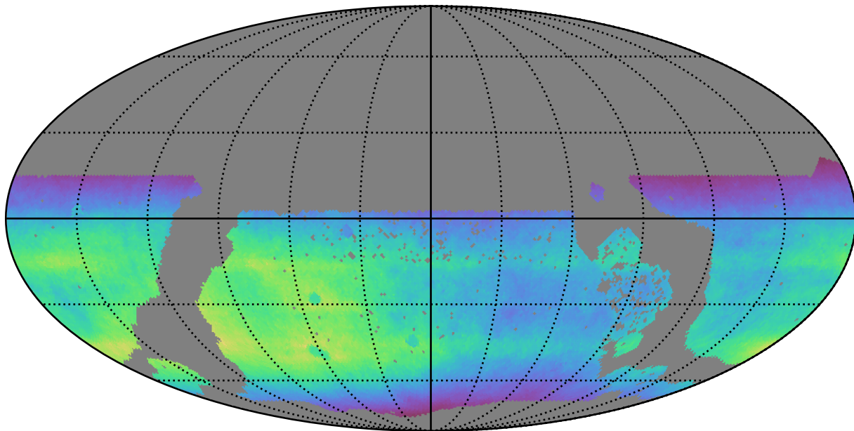
ddf_acor_sf15_lsf20_lsr20_v3.4_10yrs WFD all bands: Normalized Teff
