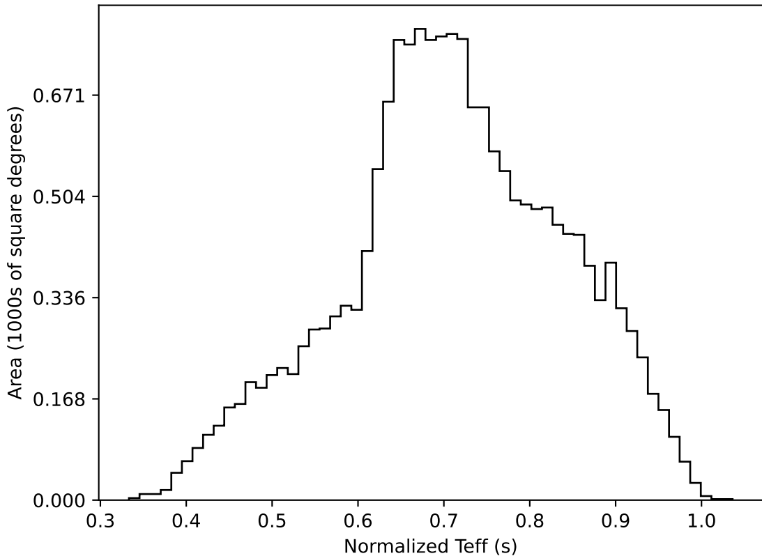
ddf_acor_sf15_lsf20_lsr20_v3.4_10yrs WFD all bands: Normalized Teff
