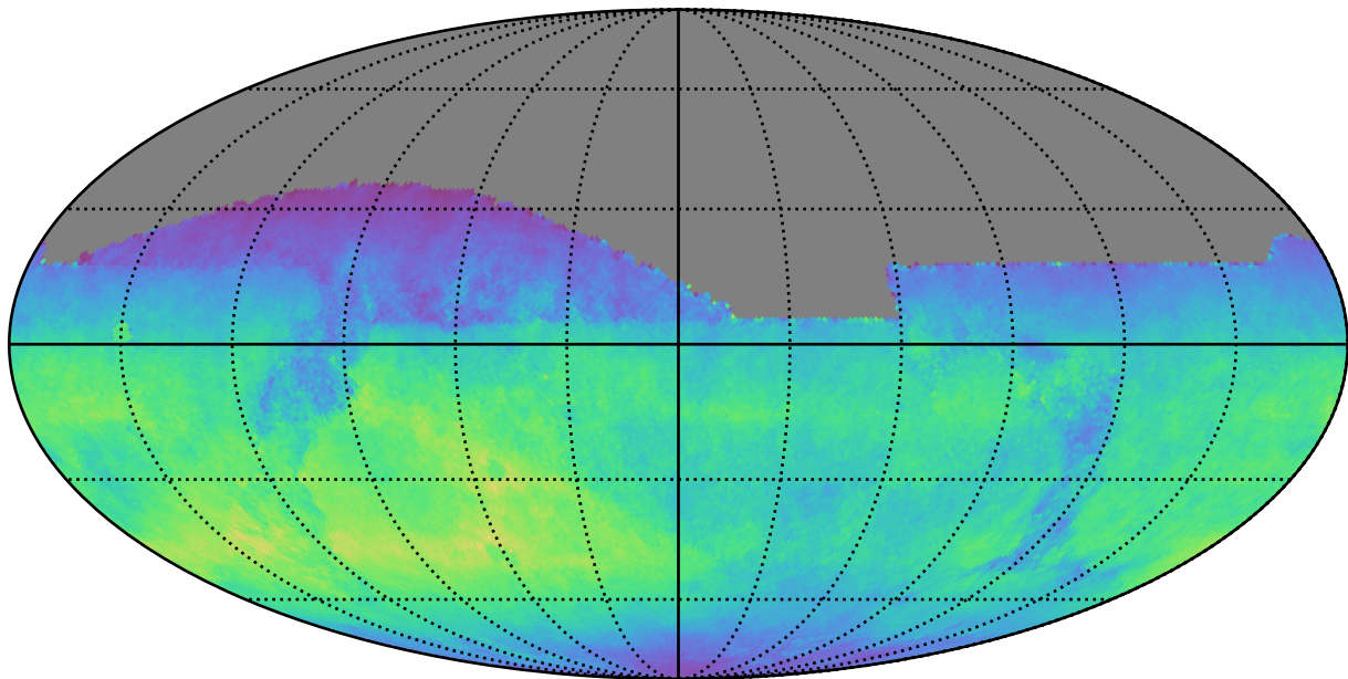
ddf_acor_sf15_lsf20_lsr20_v3.4_10yrs All sky z band: Normalized Teff
