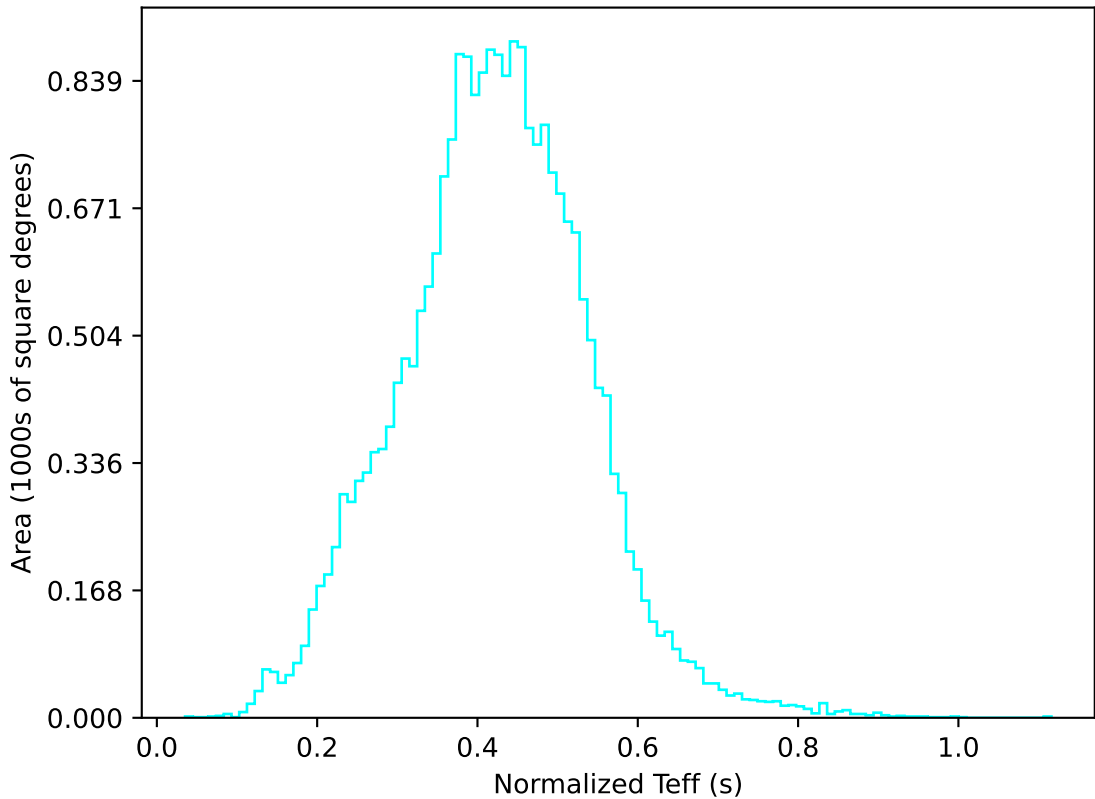
ddf_acor_sf15_lsf20_lsr20_v3.4_10yrs All sky u band: Normalized Teff
