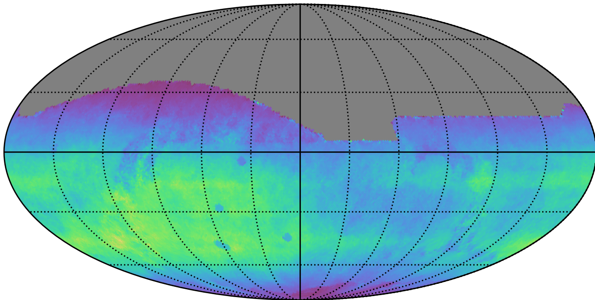
ddf_acor_sf15_lsf20_lsr20_v3.4_10yrs All sky r band: Normalized Teff
