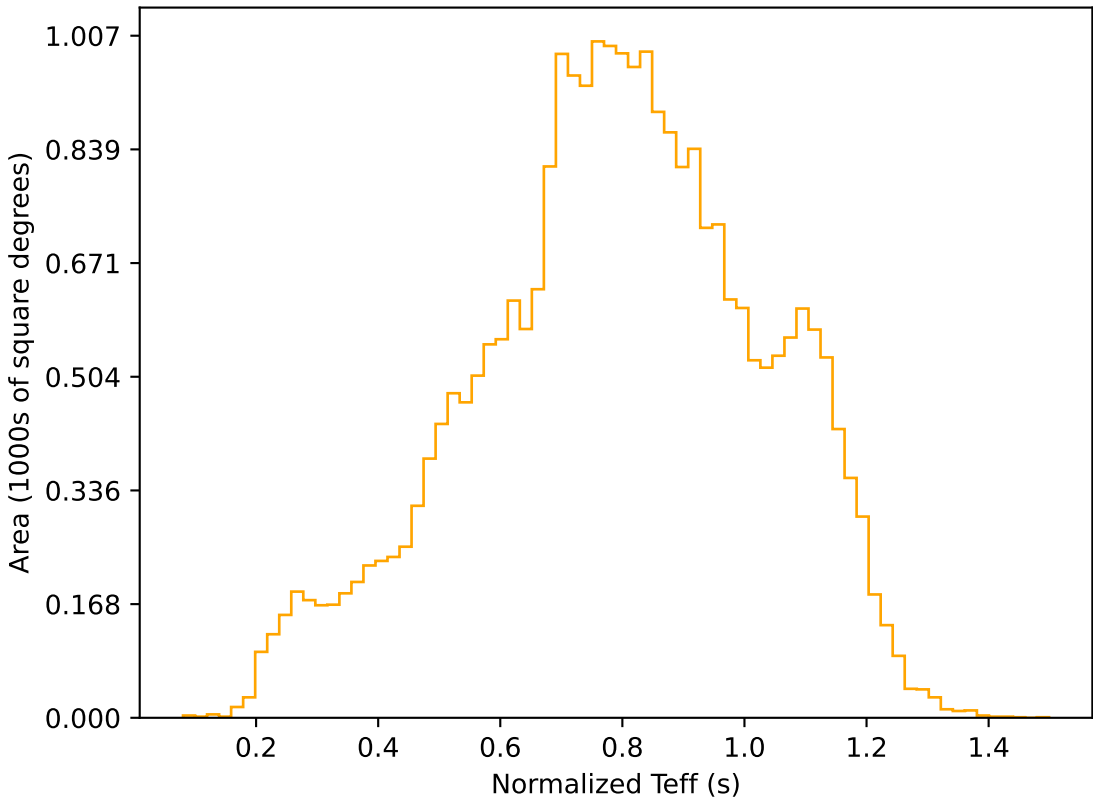
ddf_acor_sf15_lsf20_lsr20_v3.4_10yrs All sky r band: Normalized Teff
