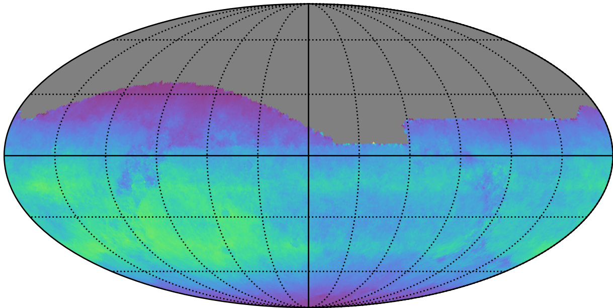
ddf_acor_sf15_lsf20_lsr20_v3.4_10yrs All sky i band: Normalized Teff
