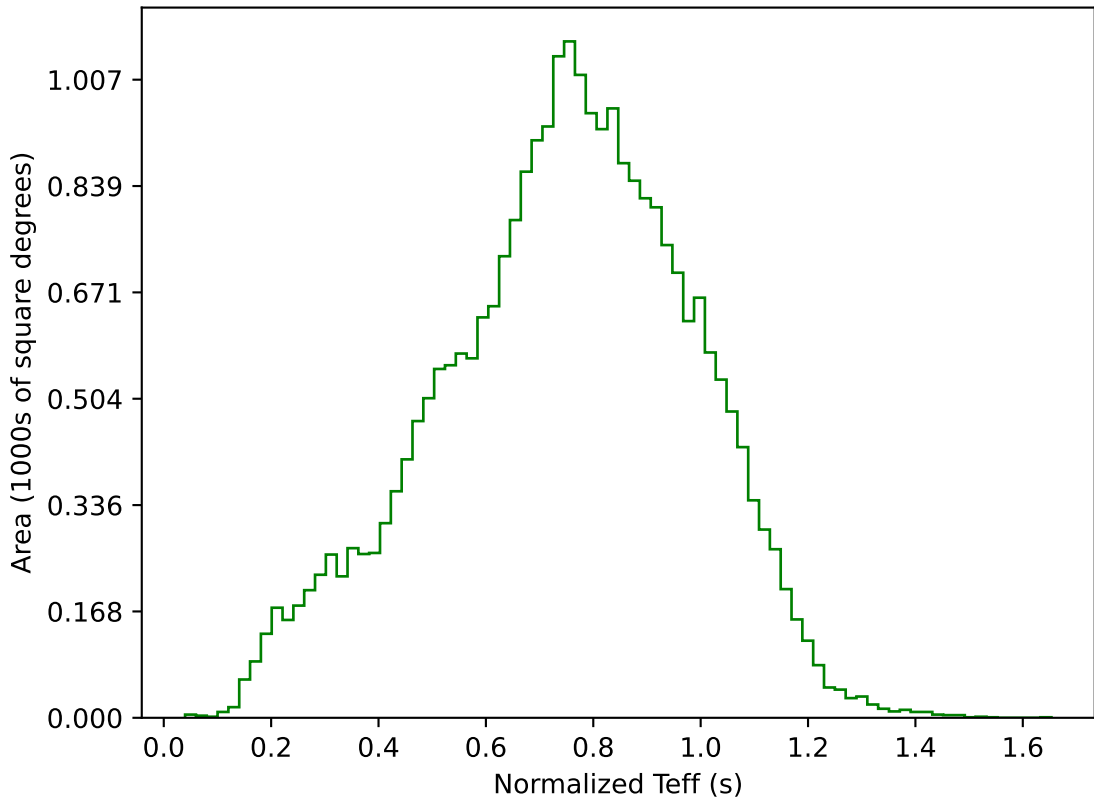
ddf_acor_sf15_lsf20_lsr20_v3.4_10yrs All sky g band: Normalized Teff
