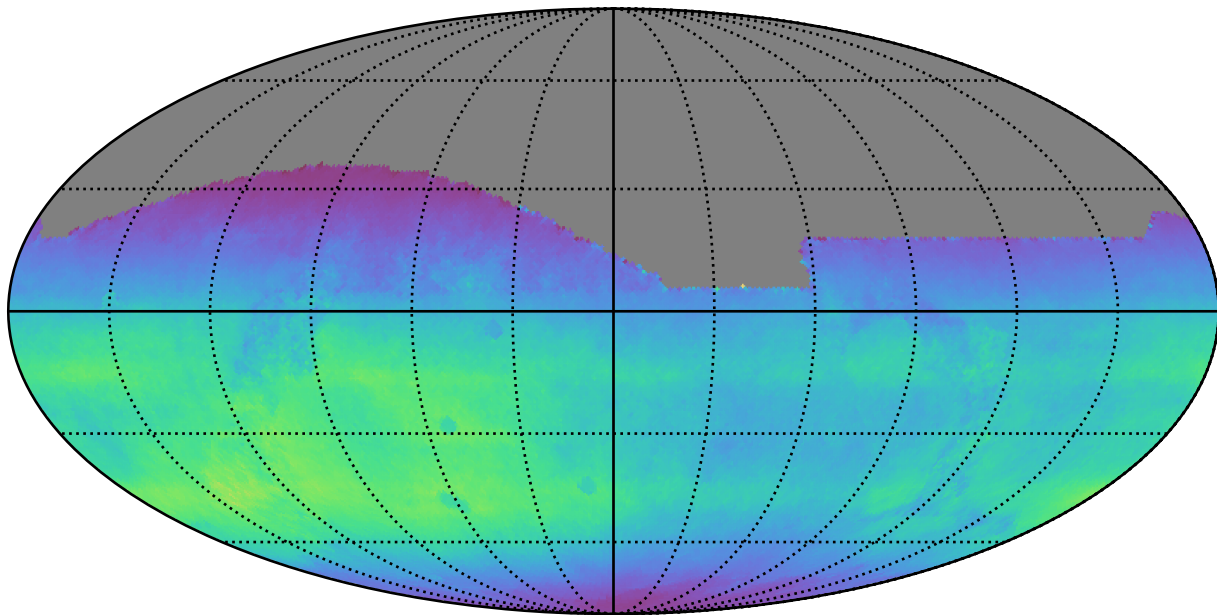
ddf_acor_sf15_lsf20_lsr20_v3.4_10yrs All sky all bands: Normalized Teff
