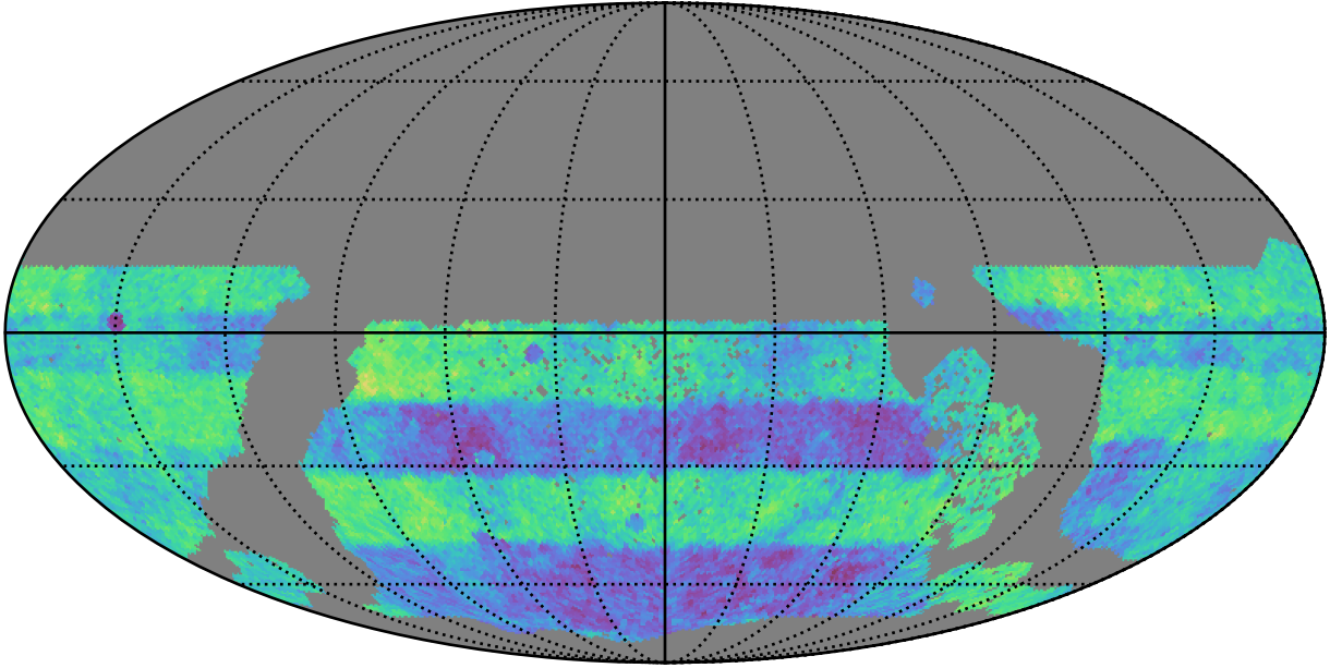
ddf_acor_sf15_lsf20_lsr20_v3.4_10yrs WFD: Normalized Proper Motion Uncert @ 24.0
