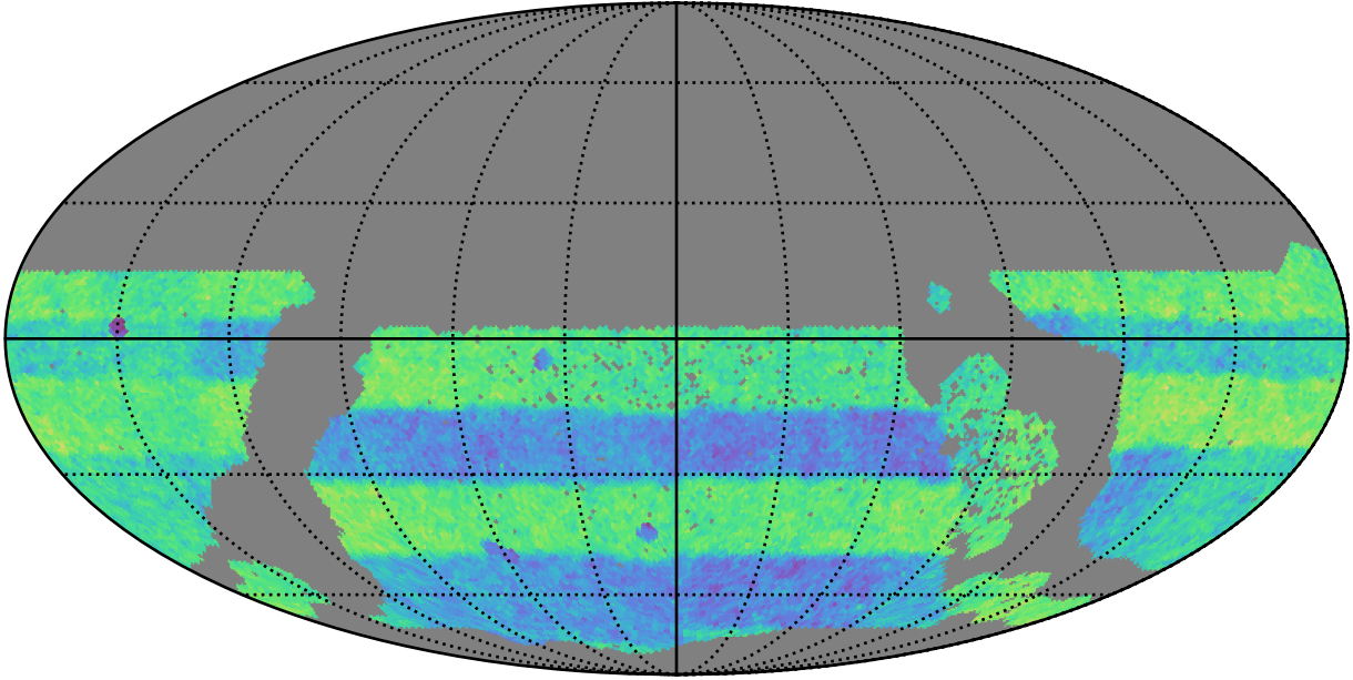
ddf_acor_sf15_lsf20_lsr20_v3.4_10yrs WFD: Normalized Proper Motion Uncert @ 20.5
