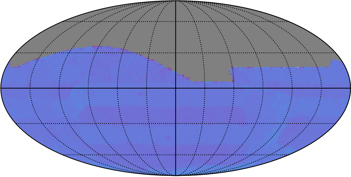
ddf_acor_sf15_lsf20_lsr20_v3.4_10yrs All sky: Normalized Proper Motion Uncert @ 20.5
