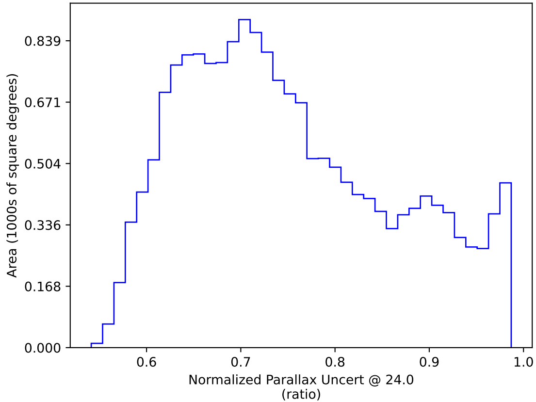
ddf_acor_sf15_lsf20_lsr20_v3.4_10yrs WFD: Normalized Parallax Uncert @ 24.0
