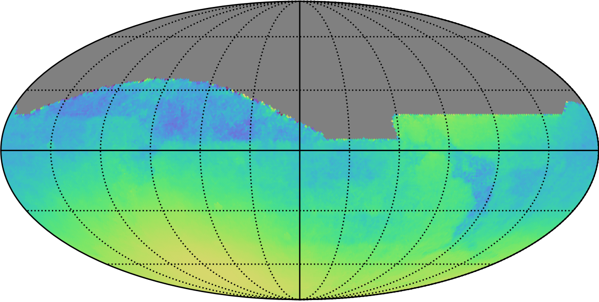
ddf_acor_sf15_lsf20_lsr20_v3.4_10yrs All sky: Normalized Parallax Uncert @ 24.0
