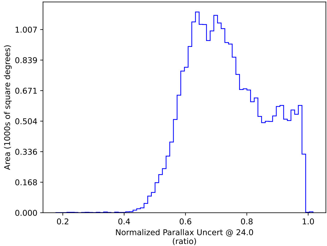
ddf_acor_sf15_lsf20_lsr20_v3.4_10yrs All sky: Normalized Parallax Uncert @ 24.0
