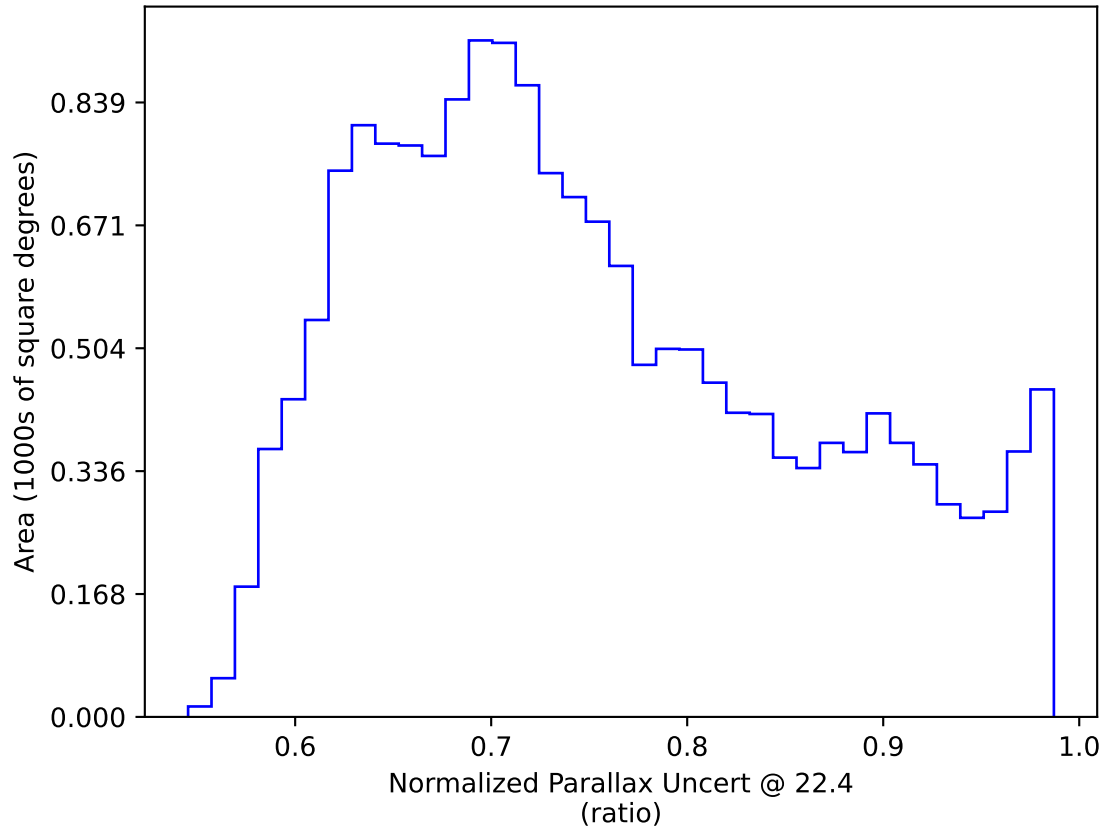
ddf_acor_sf15_lsf20_lsr20_v3.4_10yrs WFD: Normalized Parallax Uncert @ 22.4
