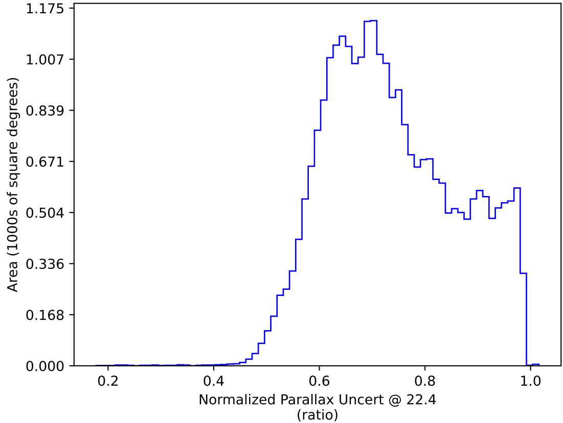
ddf_acor_sf15_lsf20_lsr20_v3.4_10yrs All sky: Normalized Parallax Uncert @ 22.4
