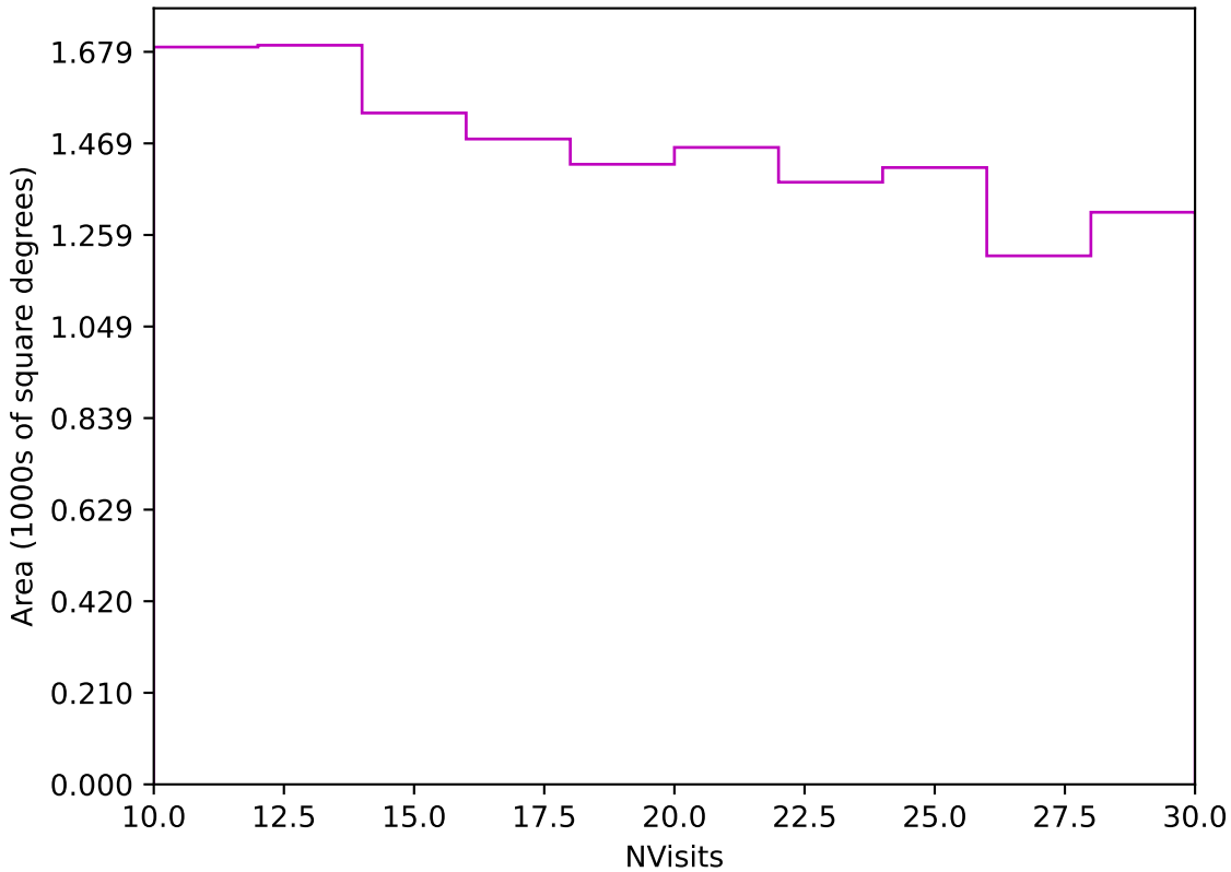
ddf_acor_sf15_lsf20_lsr20_v3.4_10yrs Yr 3-4 z band: NVisits
