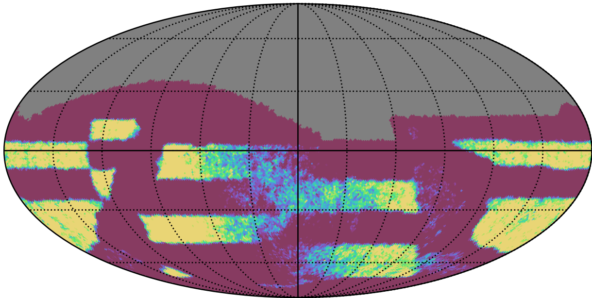
ddf_acor_sf15_lsf20_lsr20_v3.4_10yrs Yr 3-4 all bands: NVisits
