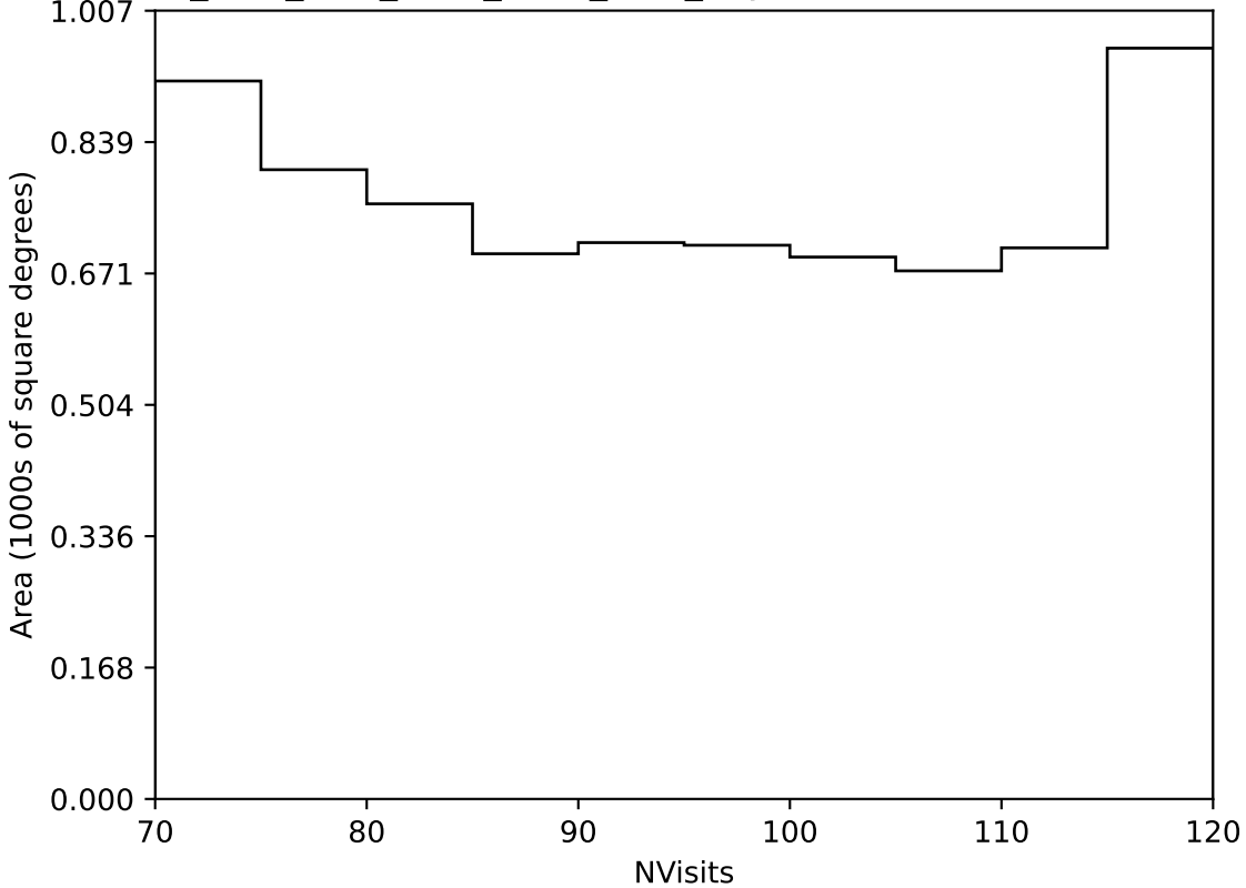
ddf_acor_sf15_lsf20_lsr20_v3.4_10yrs Yr 3-4 all bands: NVisits
