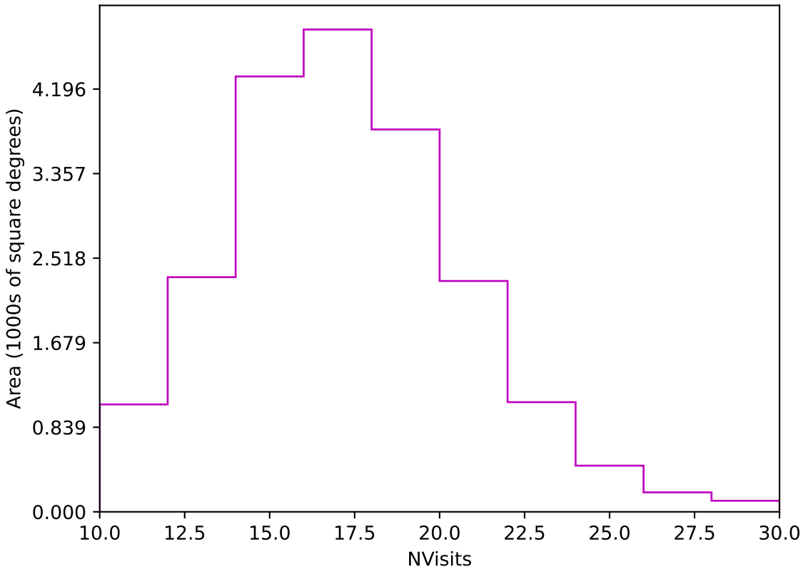
ddf_acor_sf15_lsf20_lsr20_v3.4_10yrs Yr 1 z band: NVisits
