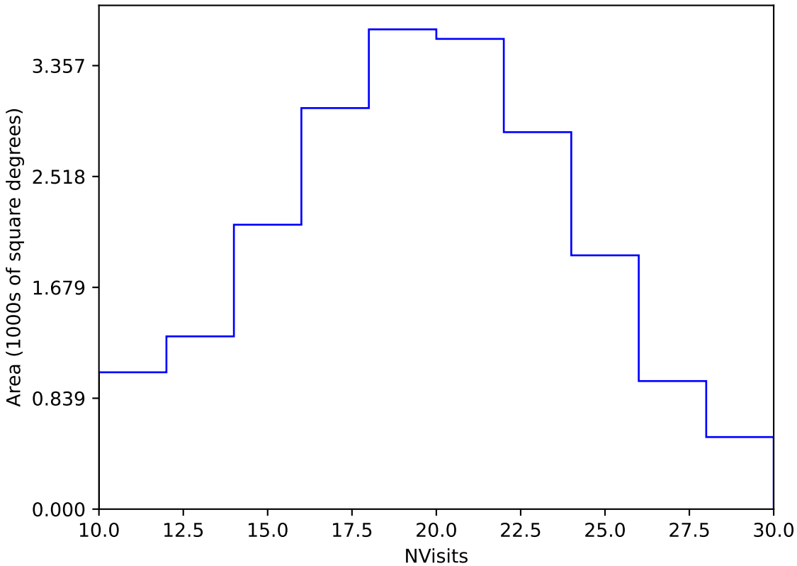
ddf_acor_sf15_lsf20_lsr20_v3.4_10yrs Yr 1 y band: NVisits
