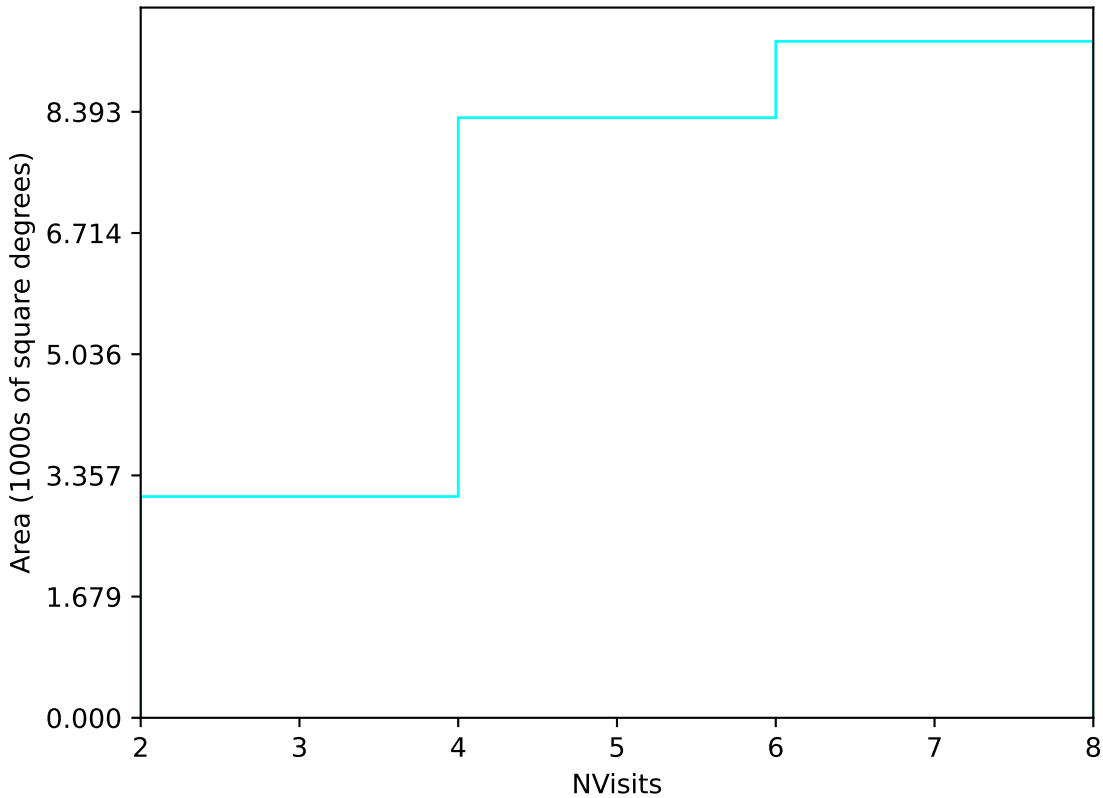
ddf_acor_sf15_lsf20_lsr20_v3.4_10yrs Yr 1 u band: NVisits
