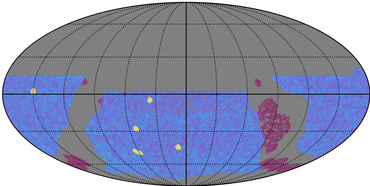
ddf_acor_sf15_lsf20_lsr20_v3.4_10yrs WFD y band: NVisits
