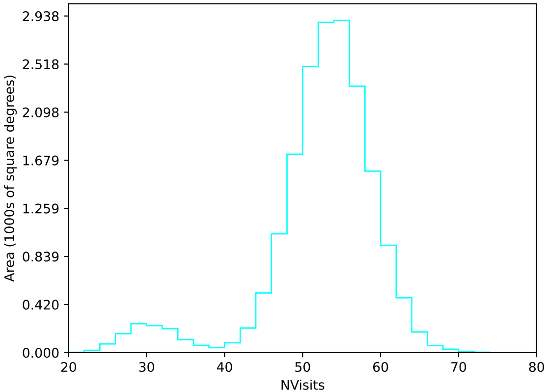
ddf_acor_sf15_lsf20_lsr20_v3.4_10yrs WFD u band: NVisits
