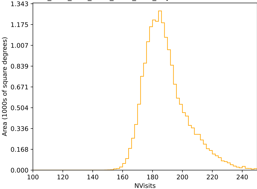
ddf_acor_sf15_lsf20_lsr20_v3.4_10yrs WFD r band: NVisits
