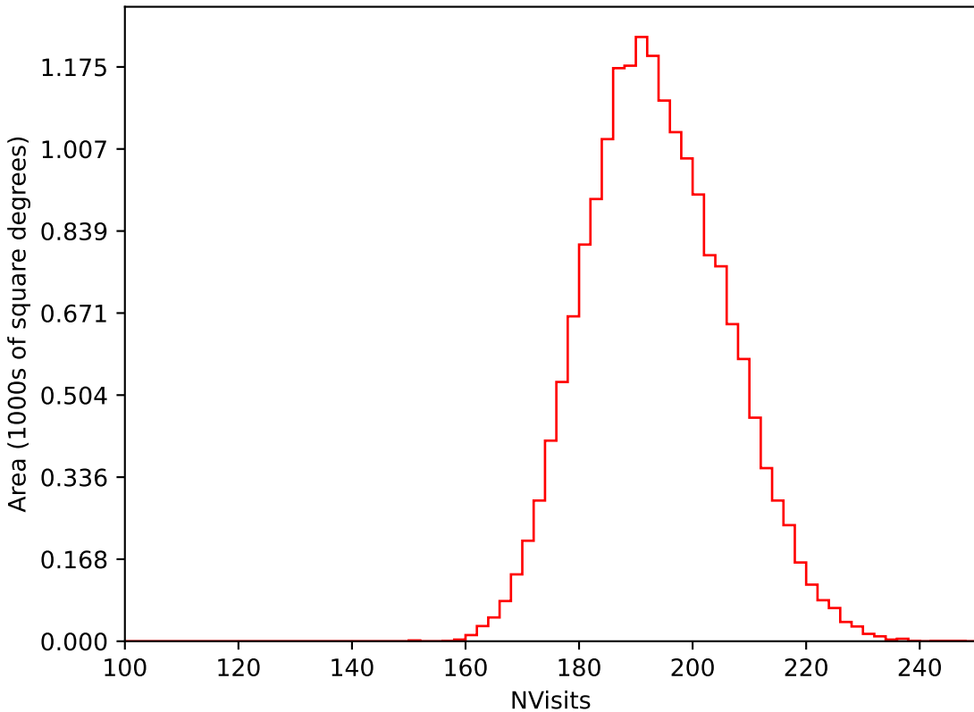
ddf_acor_sf15_lsf20_lsr20_v3.4_10yrs WFD i band: NVisits
