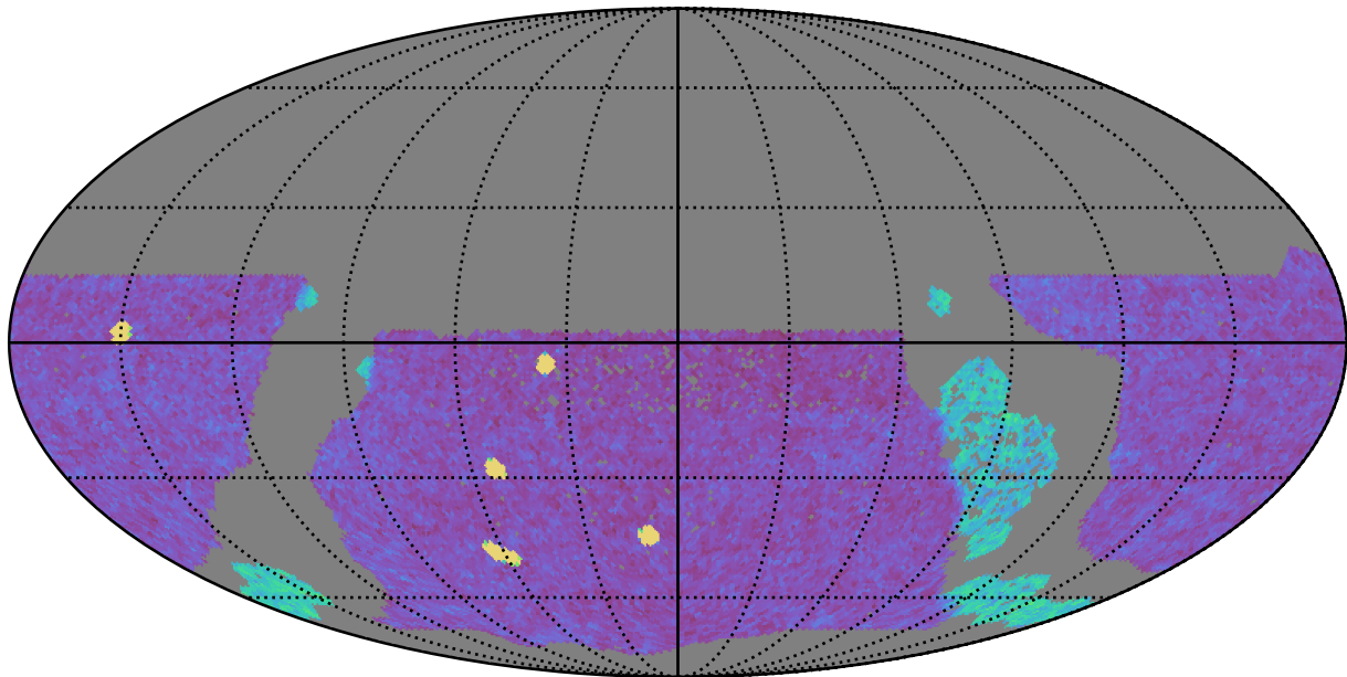
ddf_acor_sf15_lsf20_lsr20_v3.4_10yrs WFD g band: NVisits
