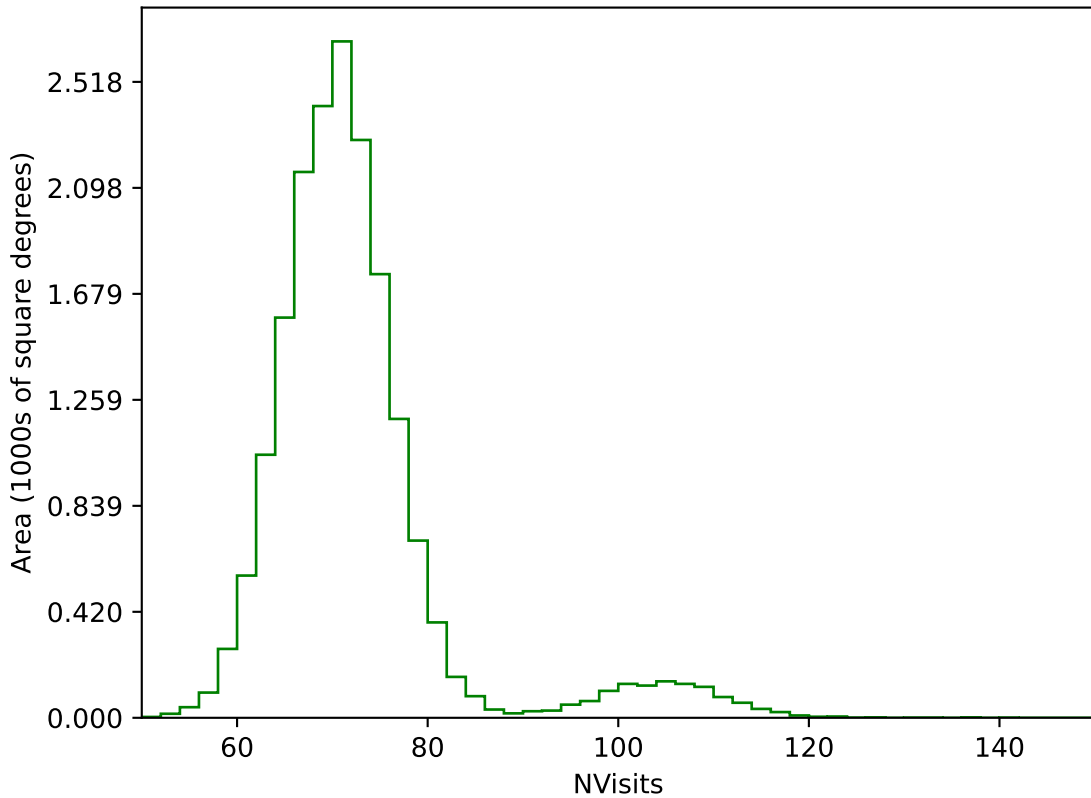
ddf_acor_sf15_lsf20_lsr20_v3.4_10yrs WFD g band: NVisits
