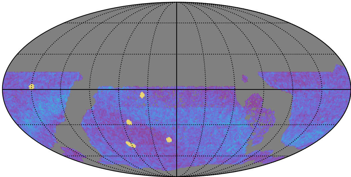
ddf_acor_sf15_lsf20_lsr20_v3.4_10yrs WFD all bands: NVisits
