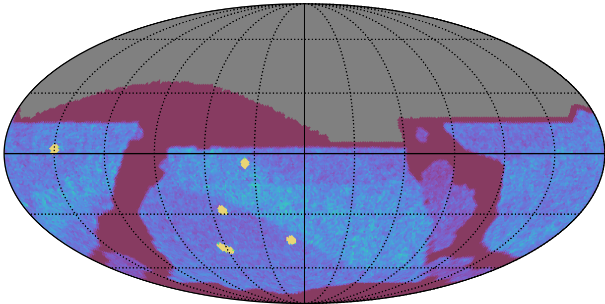
ddf_acor_sf15_lsf20_lsr20_v3.4_10yrs All sky z band: NVisits
