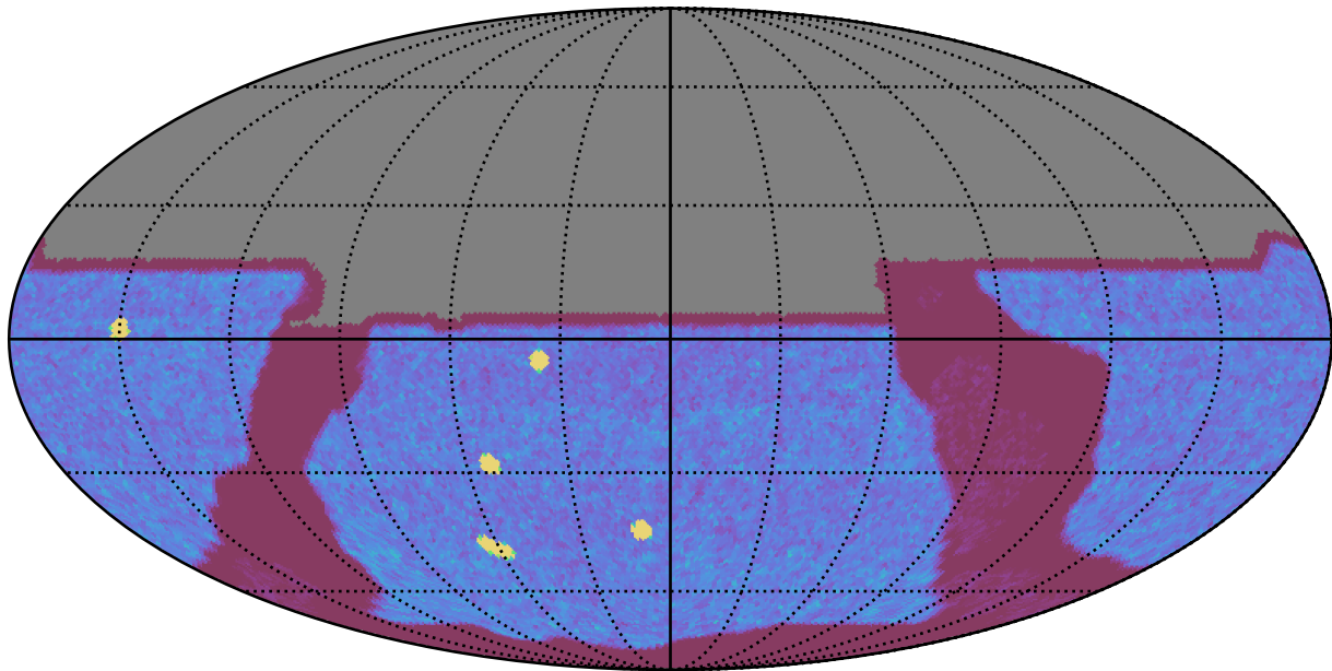
ddf_acor_sf15_lsf20_lsr20_v3.4_10yrs All sky y band: NVisits
