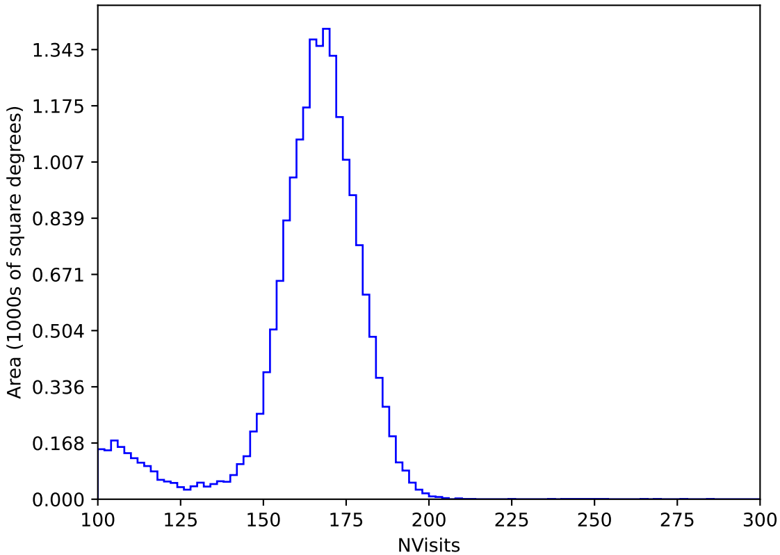
ddf_acor_sf15_ls20_lsr20_v3.4_10yrs All sky y band: NVisits
