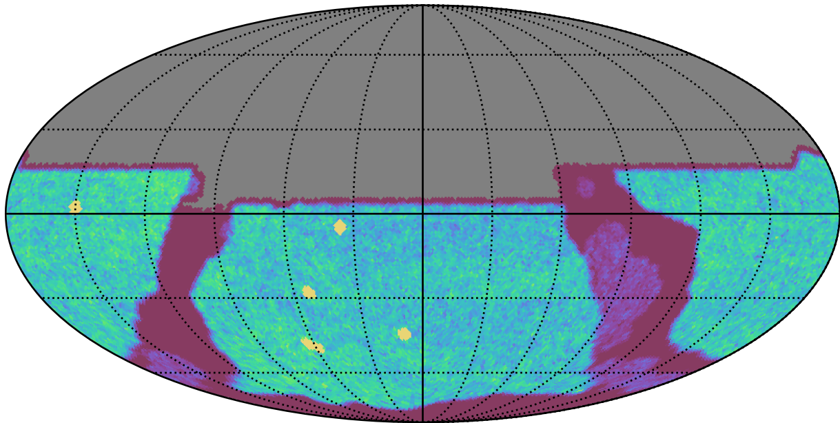
ddf_acor_sf15_lsf20_lsr20_v3.4_10yrs All sky u band: NVisits
