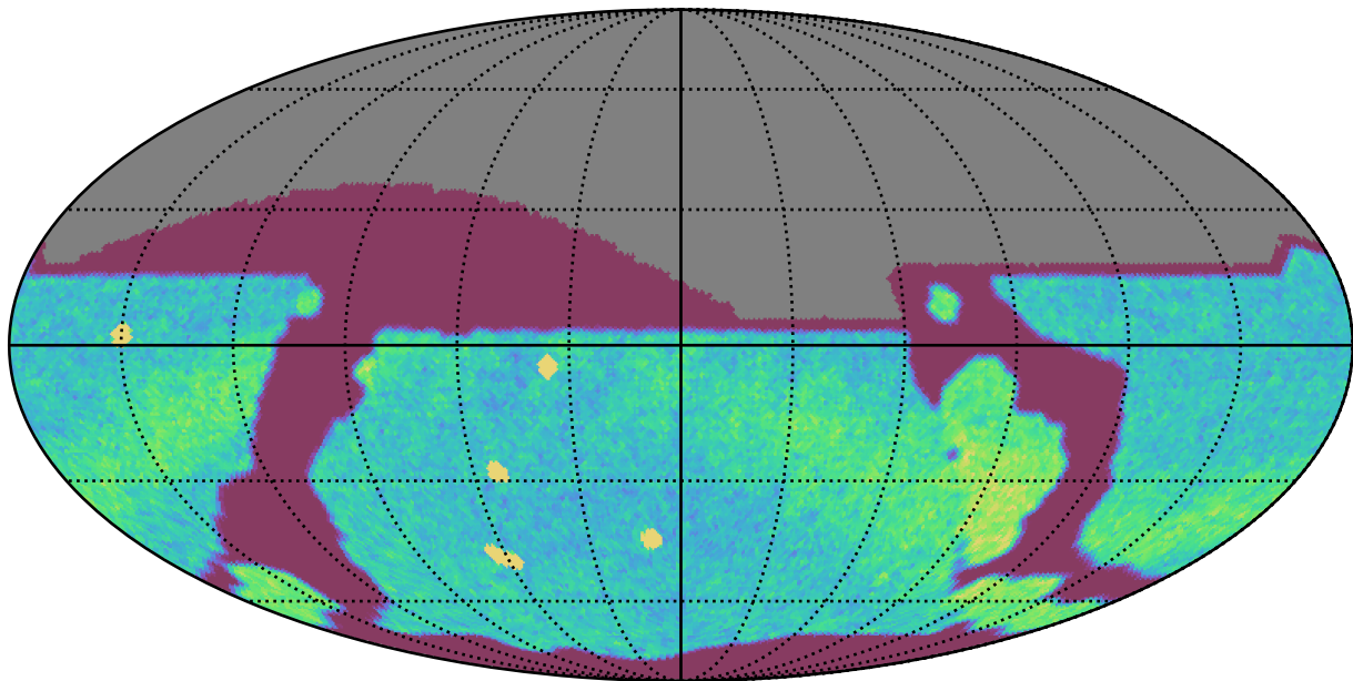
ddf_acor_sf15_lsf20_lsr20_v3.4_10yrs All sky r band: NVisits
