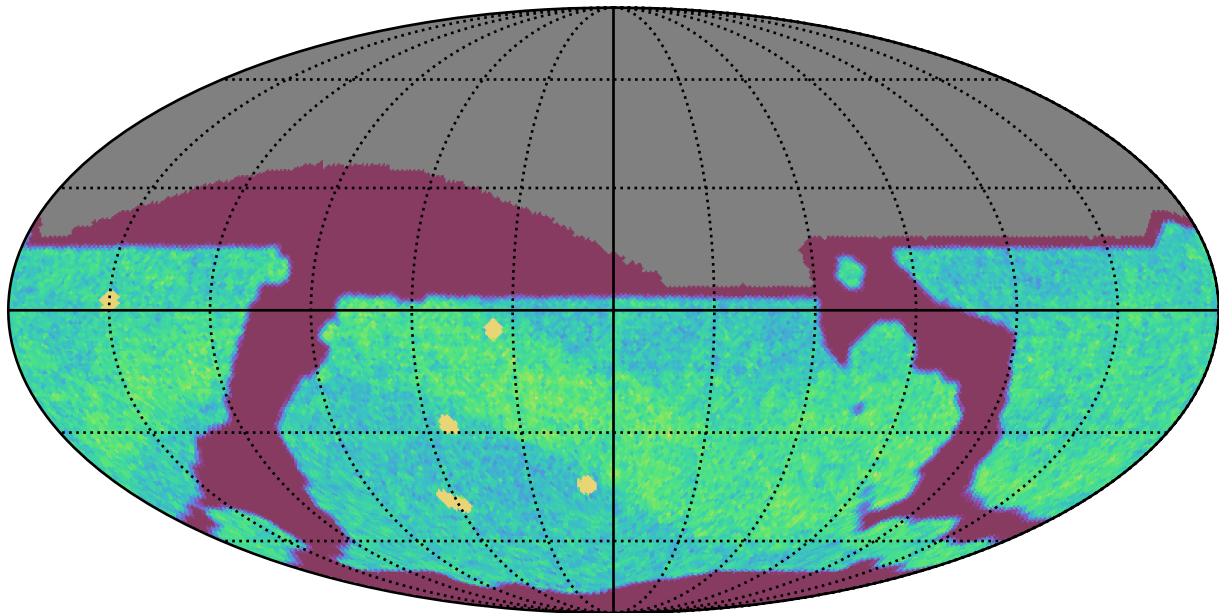
ddf_acor_sf15_lsf20_lsr20_v3.4_10yrs All sky i band: NVisits
