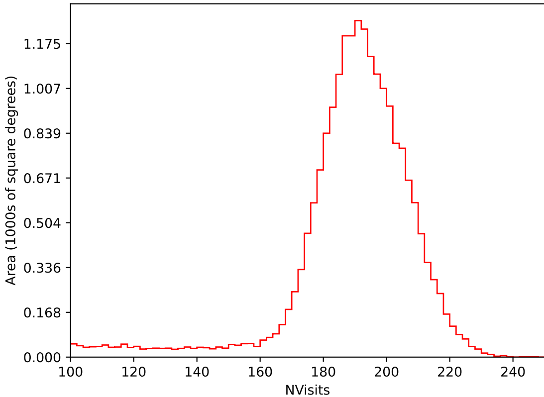
ddf_acor_sf15_lsf20_lsr20_v3.4_10yrs All sky i band: NVisits
