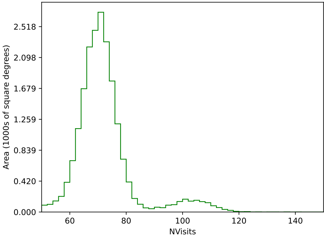
ddf_acor_sf15_lsf20_lsr20_v3.4_10yrs All sky g band: NVisits
