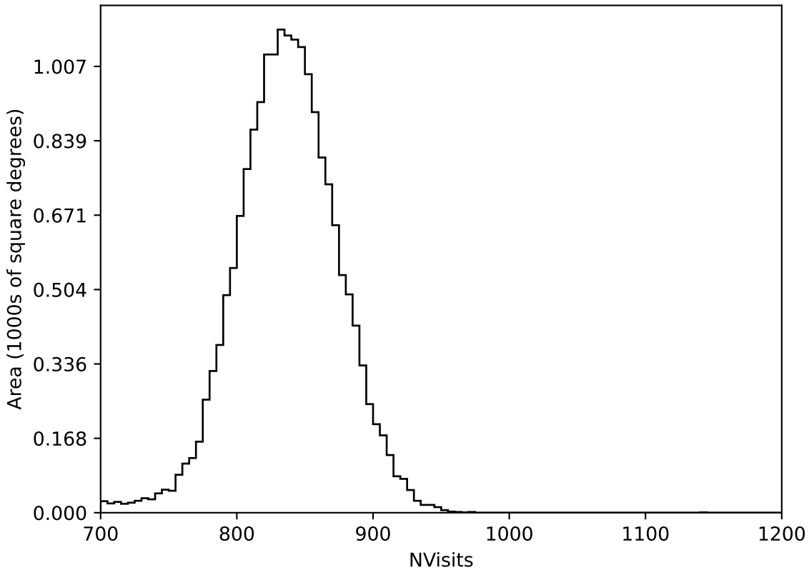
ddf_acor_sf15_lsf20_lsr20_v3.4_10yrs All sky all bands: NVisits
