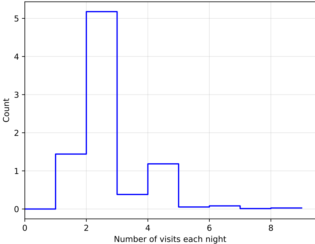
ddf_acor_sf15_lsf20_lsr20_v3.4_10yrs WFD: NVisitsPerNight 1e6
